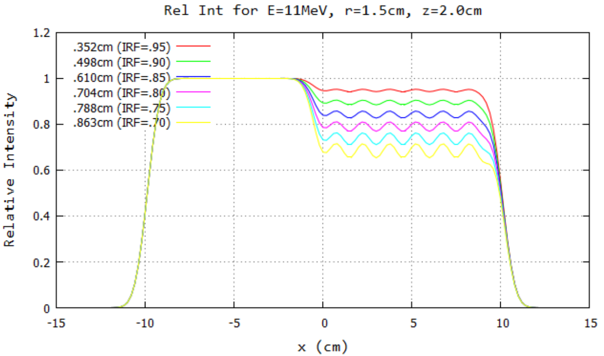
Figure B.55: Profile for 11 MeV and 103 cm SSD at y=0\text{cm} 20x20 half-blocked field. The computed island block diameter for 0.70, 0.75, 0.80, 0.85, 0.90, and 0.95 IRF values are listed in each plot's inserted key.
