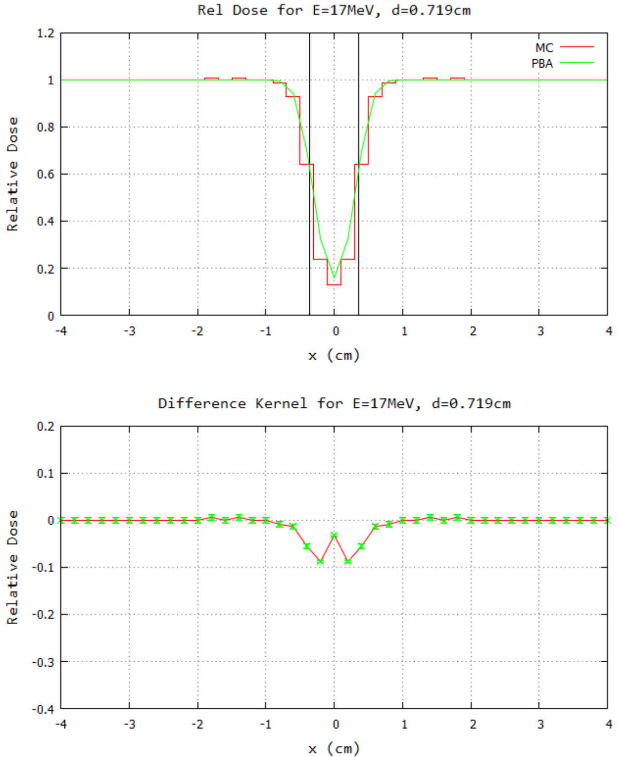
Figure A.17: Monte Carlo central axis block profile and kernel: monoenergetic 17 MeV beam with a central axis block of diameter d=0.719 cm at depth z=0.5 cm with air gap g=5.0 cm. (top) Crossplane intensity profile ( y=0 ) for MC and PBA. Upright block lines indicate the edges of the block. (bottom) MC-PBA difference kernel with error bars.
