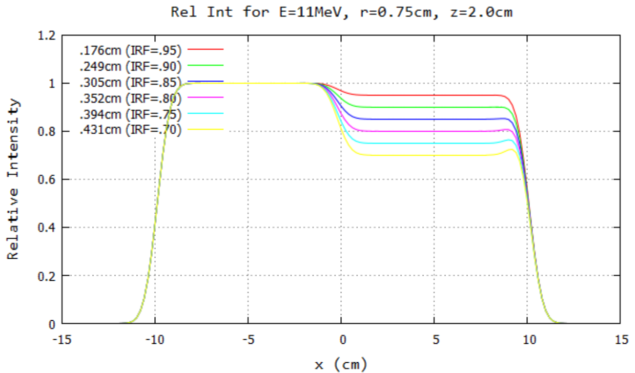
Figure B.52: Profile for 11 MeV and 103 cm SSD at y=0 cm 20x20 half-blocked field. The computed island block diameter for 0.70, 0.75, 0.80, 0.85, 0.90, and 0.95 IRF values are listed in each plot's inserted key.
