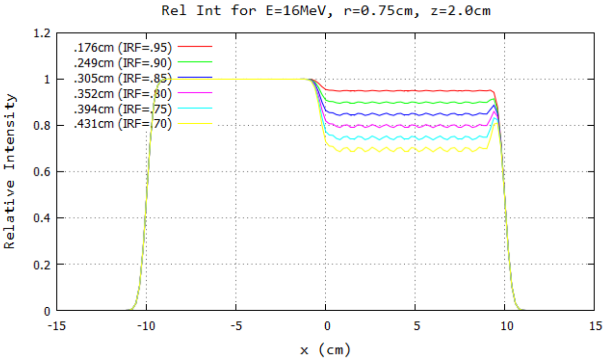
Figure B.27: Profile for 16 MeV and 100 cm SSD at y=0 cm 20x20 half-blocked field. The computed island block diameter for 0.70, 0.75, 0.80, 0.85, 0.90, and 0.95 IRF values are listed in each plot's inserted key.
