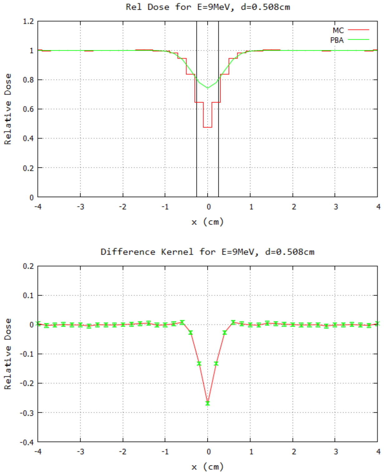
Figure A.4: Monte Carlo central axis block profile and kernel: monoenergetic 9 MeV beam with a central axis block of diameter d=0.508\text{cm} at depth z=0.5\text{cm} with air gap g=5.0\text{cm} . (top) Crossplane intensity profile ( y=0 ) for MC and PBA. Upright block lines indicate the edges of the block. (bottom) MC-PBA difference kernel with error bars.
