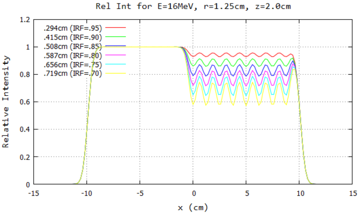
Figure B.64: Profile for 16 MeV and 103 cm SSD at y=0\text{cm} 20x20 half-blocked field. The computed island block diameter for 0.70, 0.75, 0.80, 0.85, 0.90, and 0.95 IRF values are listed in each plot's inserted key.
