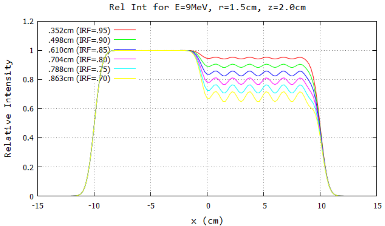
Figure B.10: Profile for 9 MeV and 100 cm SSD at y=0\text{cm} 20x20 half-blocked field. The computed island block diameter for 0.70, 0.75, 0.80, 0.85, 0.90, and 0.95 IRF values are listed in each plot's inserted key.
