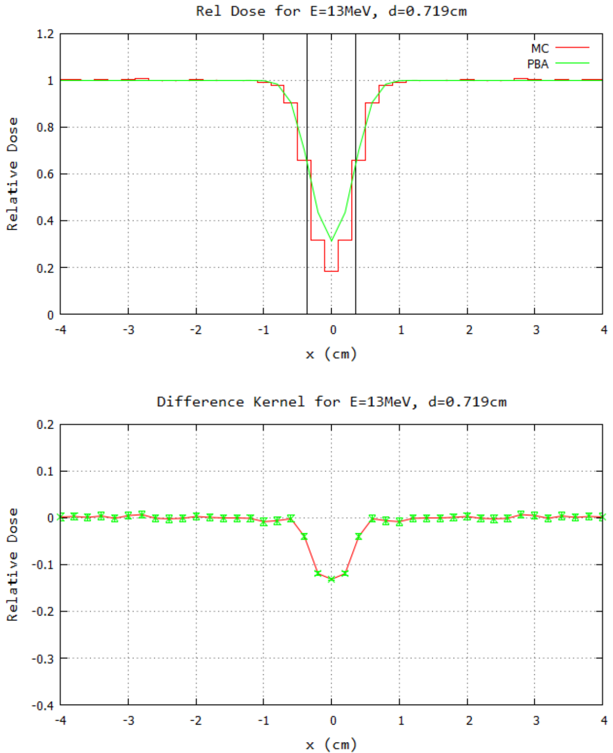
Figure A.11: Monte Carlo central axis block profile and kernel: monoenergetic 13 MeV beam with a central axis block of diameter d=0.719 cm at depth z=0.5 cm with air gap g=5.0 cm. (top) Crossplane intensity profile ( y=0 ) for MC and PBA. Upright block lines indicate the edges of the block. (bottom) MC-PBA difference kernel with error bars.
