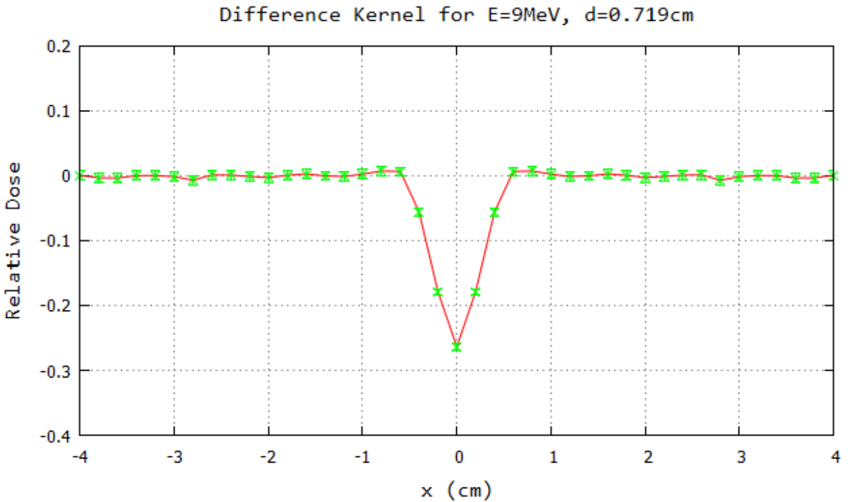
Figure A.5: Monte Carlo central axis block profile and kernel: monoenergetic 9 MeV beam with a central axis block of diameter d=0.719\text{cm} at depth z=0.5\text{cm} with air gap g=5.0\text{cm} . (top) Crossplane intensity profile ( y=0 ) for MC and PBA. Upright block lines indicate the edges of the block. (bottom) MC-PBA difference kernel with error bars.
