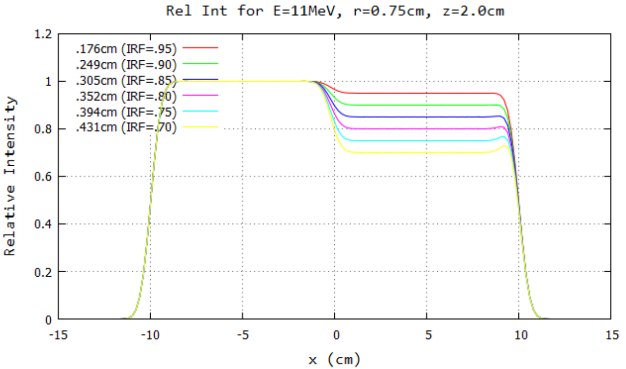
Figure B.17: Profile for 11 MeV and 100 cm SSD at y=0 cm 20x20 half-blocked field. The computed island block diameter for 0.70, 0.75, 0.80, 0.85, 0.90, and 0.95 IRF values are listed in each plot's inserted key.
