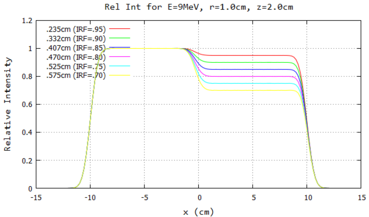
Figure B.8: Profile for 9 MeV and 100 cm SSD at y=0 cm 20x20 half-blocked field. The computed island block diameter for 0.70, 0.75, 0.80, 0.85, 0.90, and 0.95 IRF values are listed in each plot's inserted key.
