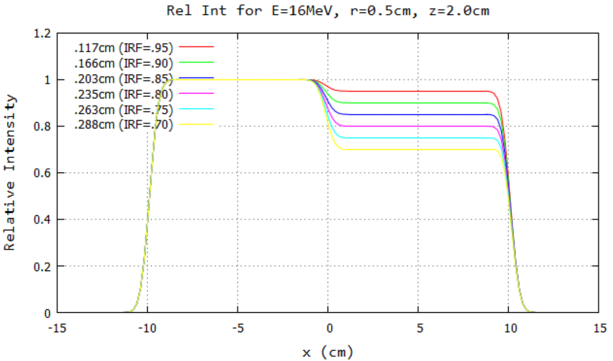
Figure 3.6: Profiles at y=0\text{cm} for 16 MeV, 20\times 20 half-blocked field ( r=0.5\text{cm} ), 100 cm SSD: z=0.5\text{cm} (top) and z=2.0\text{cm} (bottom). The computed island block diameter for 0.70, 0.75, 0.80, 0.85, 0.90, and 0.95 IRF values are listed in each plot's inserted key.
