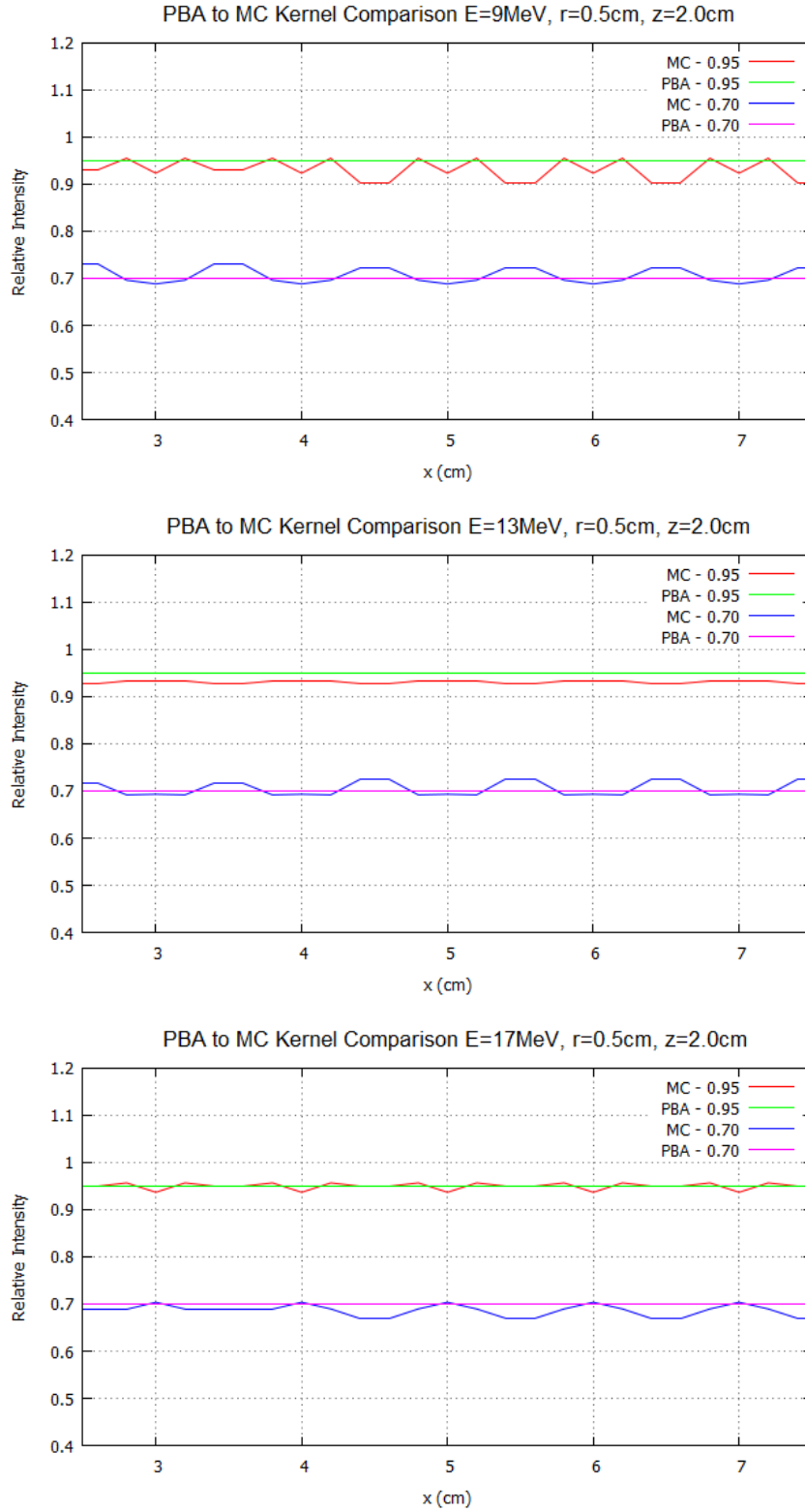
Figure 2.12: Off-axis profile for 9, 13, and 17 MeV beam at 100 cm SSD, IRF=0.95 ( d=.117\text{cm} ) and IRF=0.70 ( d=.288\text{cm} ), through y=0\text{cm} of a 20 \times 20\text{ cm}^2 half-blocked field.
