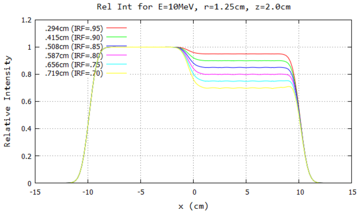
Figure B.49: Profile for 10 MeV and 103 cm SSD at y=0\text{cm} 20x20 half-blocked field. The computed island block diameter for 0.70, 0.75, 0.80, 0.85, 0.90, and 0.95 IRF values are listed in each plot's inserted key.
