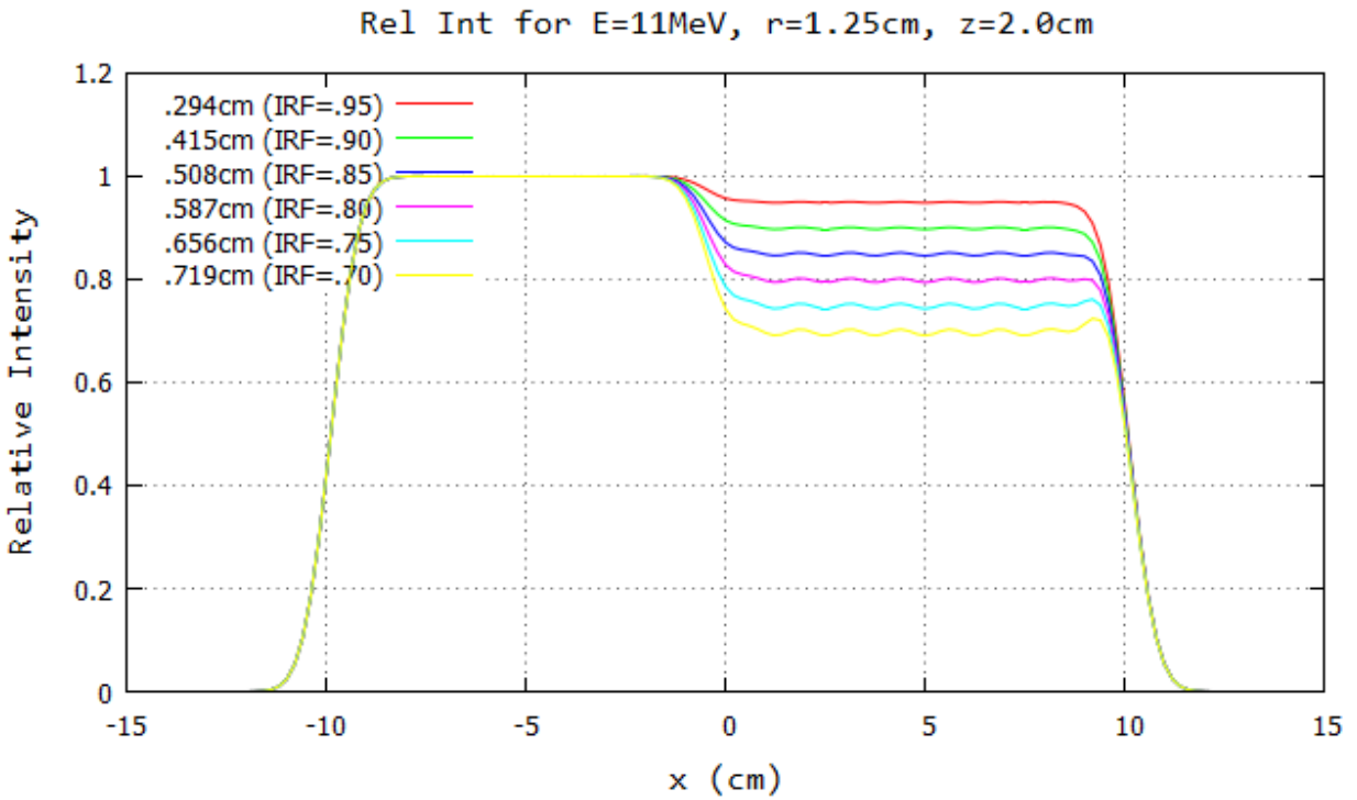
Figure B.54: Profile for 11 MeV and 103 cm SSD at y=0\text{cm} 20x20 half-blocked field. The computed island block diameter for 0.70, 0.75, 0.80, 0.85, 0.90, and 0.95 IRF values are listed in each plot's inserted key.
