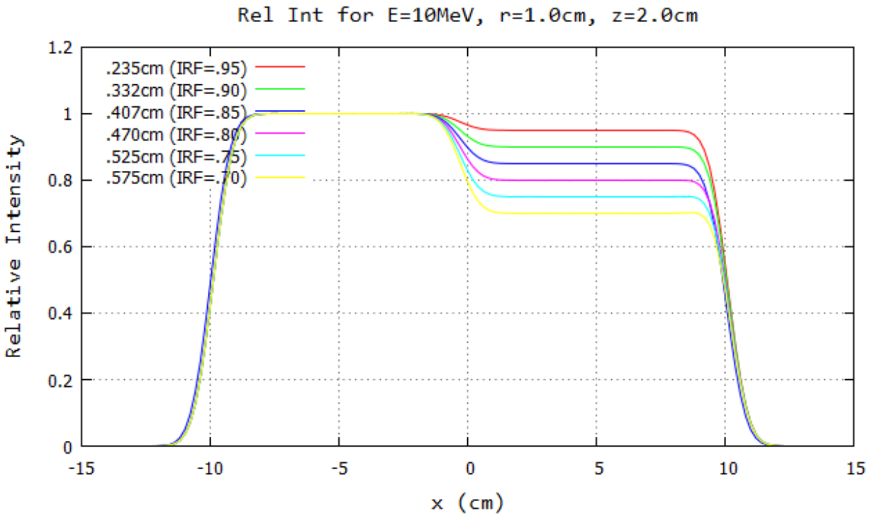
Figure B.48: Profile for 10 MeV and 103 cm SSD at y=0\text{cm} 20x20 half-blocked field. The computed island block diameter for 0.70, 0.75, 0.80, 0.85, 0.90, and 0.95 IRF values are listed in each plot's inserted key.
