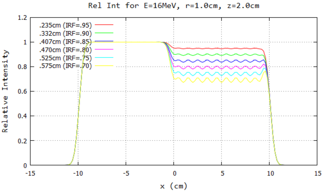
Figure B.63: Profile for 16 MeV and 103 cm SSD at y=0\text{cm} 20x20 half-blocked field. The computed island block diameter for 0.70, 0.75, 0.80, 0.85, 0.90, and 0.95 IRF values are listed in each plot's inserted key.
