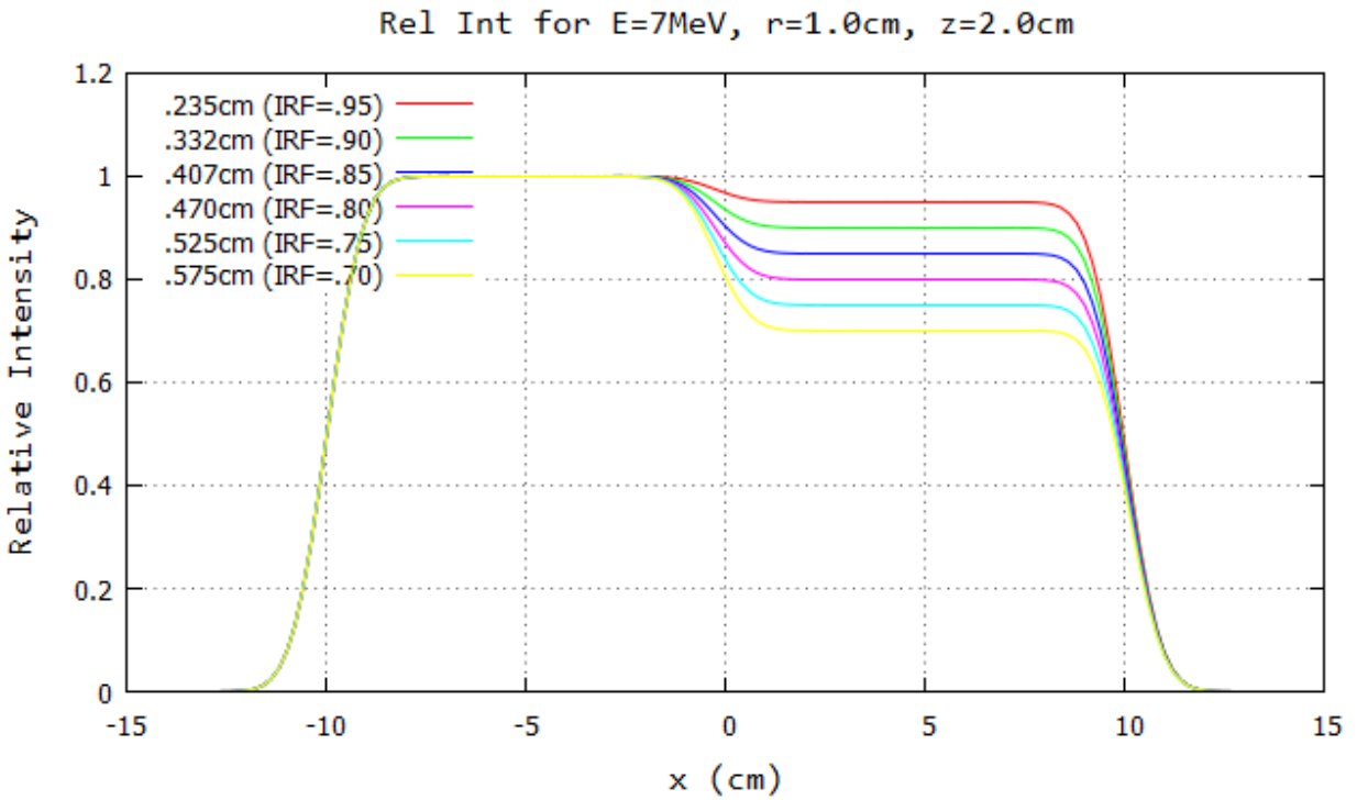
Figure B.3: Profile for 7 MeV and 100 cm SSD at y=0\text{cm} 20x20 half-blocked field. The computed island block diameter for 0.70, 0.75, 0.80, 0.85, 0.90, and 0.95 IRF values are listed in each plot's inserted key.
