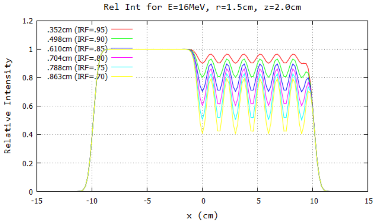
Figure 3.8: Profiles at y=0\text{cm} for 16 MeV, 20\times 20 half-blocked field ( r=1.5\text{cm} ), 100 cm SSD: z=0.5\text{cm} (top) and z=2.0\text{cm} (bottom). The computed island block diameter for 0.70, 0.75, 0.80, 0.85, 0.90, and 0.95 IRF values are listed in each plot's inserted key.
