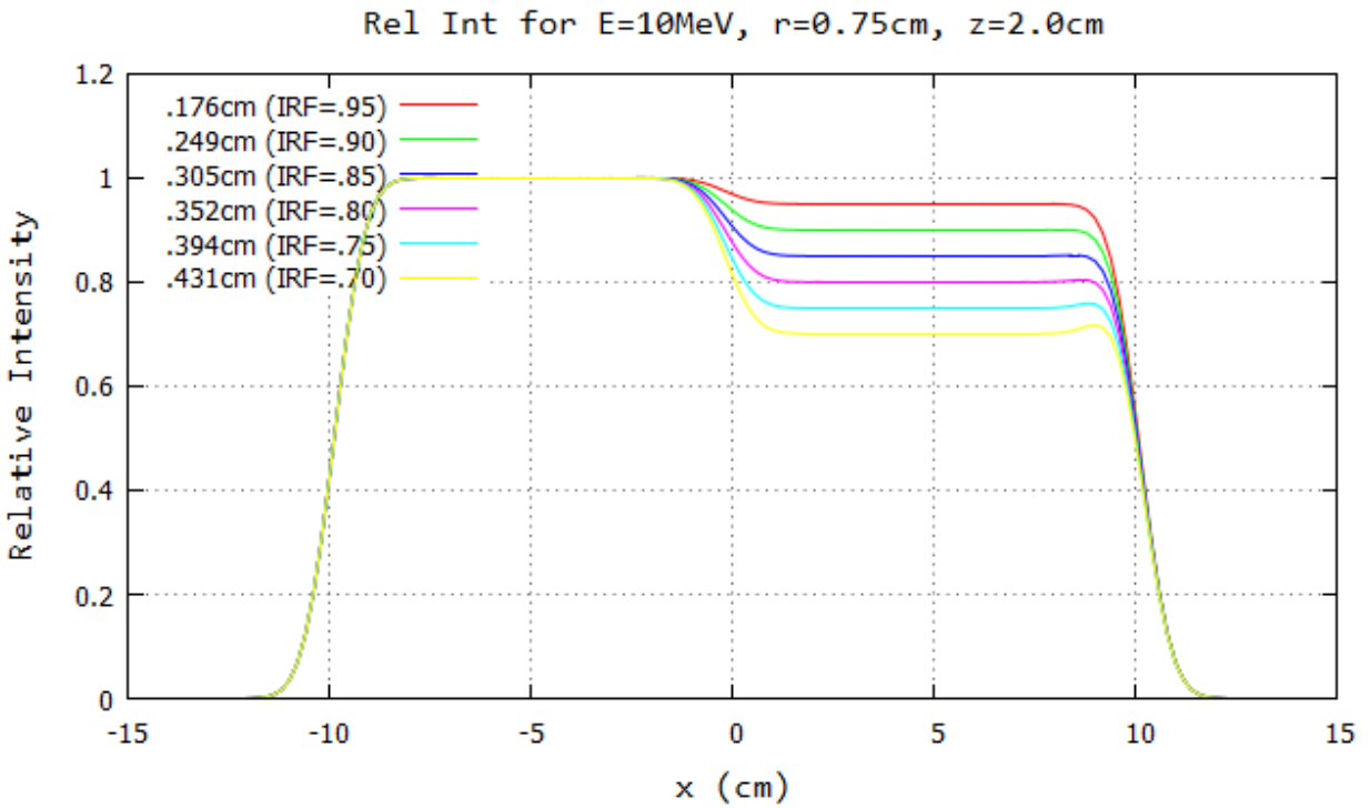
Figure B.47: Profile for 10 MeV and 103 cm SSD at y=0 cm 20x20 half-blocked field. The computed island block diameter for 0.70, 0.75, 0.80, 0.85, 0.90, and 0.95 IRF values are listed in each plot's inserted key.
