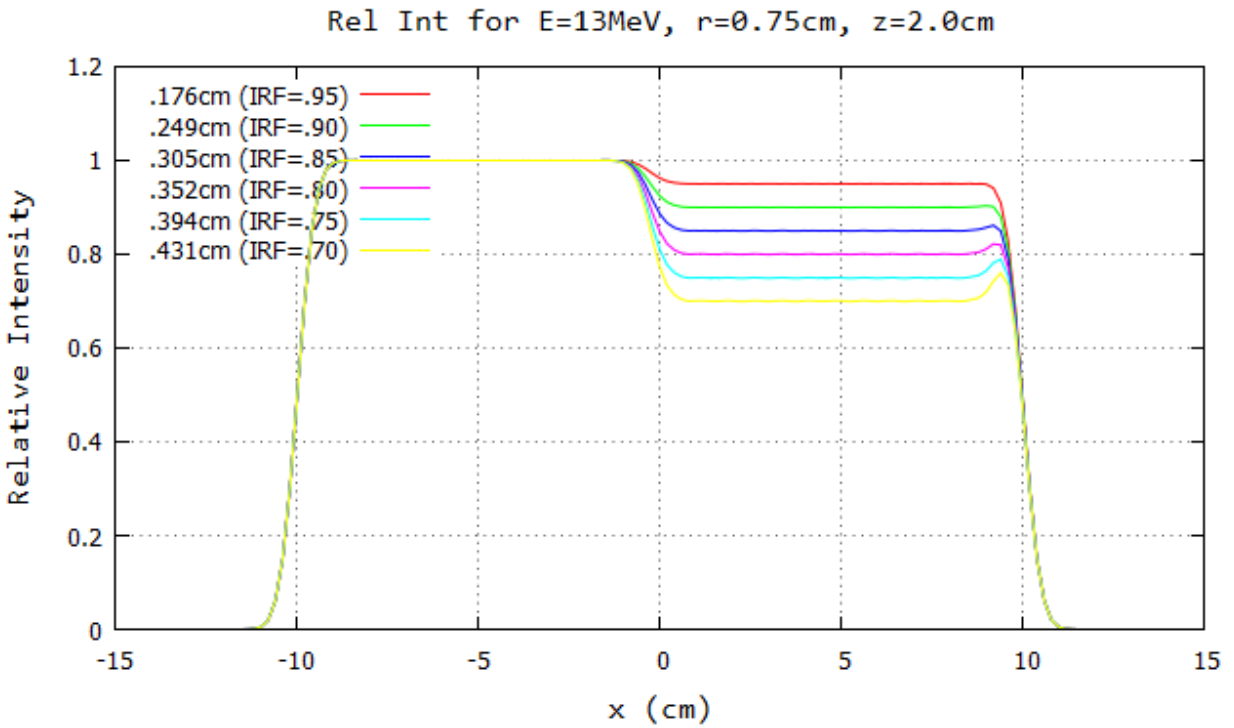
Figure B.22: Profile for 13 MeV and 100 cm SSD at y=0\text{cm} 20x20 half-blocked field. The computed island block diameter for 0.70, 0.75, 0.80, 0.85, 0.90, and 0.95 IRF values are listed in each plot's inserted key.
