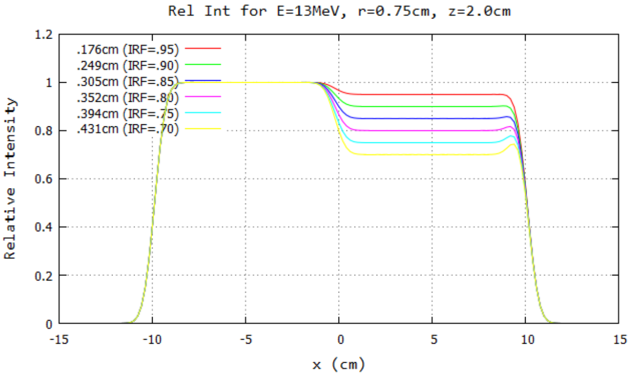
Figure B.57: Profile for 13 MeV and 103 cm SSD at y=0\text{cm} 20x20 half-blocked field. The computed island block diameter for 0.70, 0.75, 0.80, 0.85, 0.90, and 0.95 IRF values are listed in each plot's inserted key.
