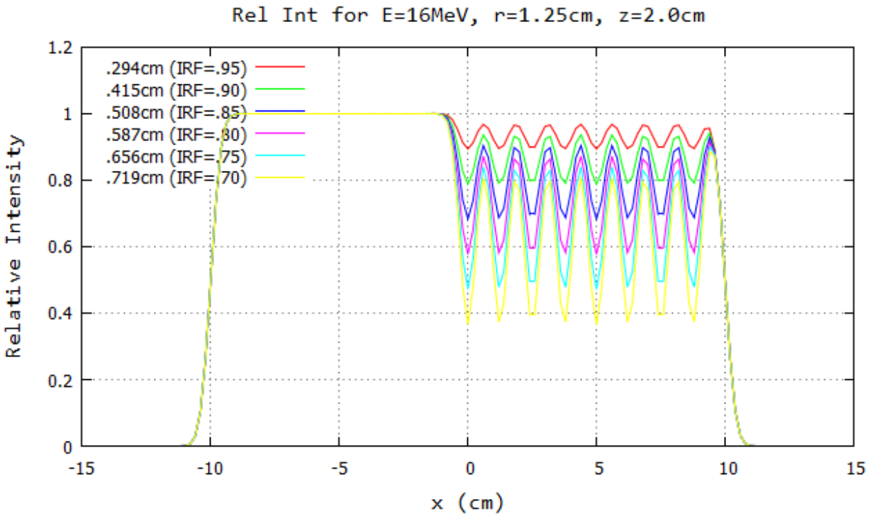
Figure B.29: Profile for 16 MeV and 100 cm SSD at y=0\text{cm} 20x20 half-blocked field. The computed island block diameter for 0.70, 0.75, 0.80, 0.85, 0.90, and 0.95 IRF values are listed in each plot's inserted key.
