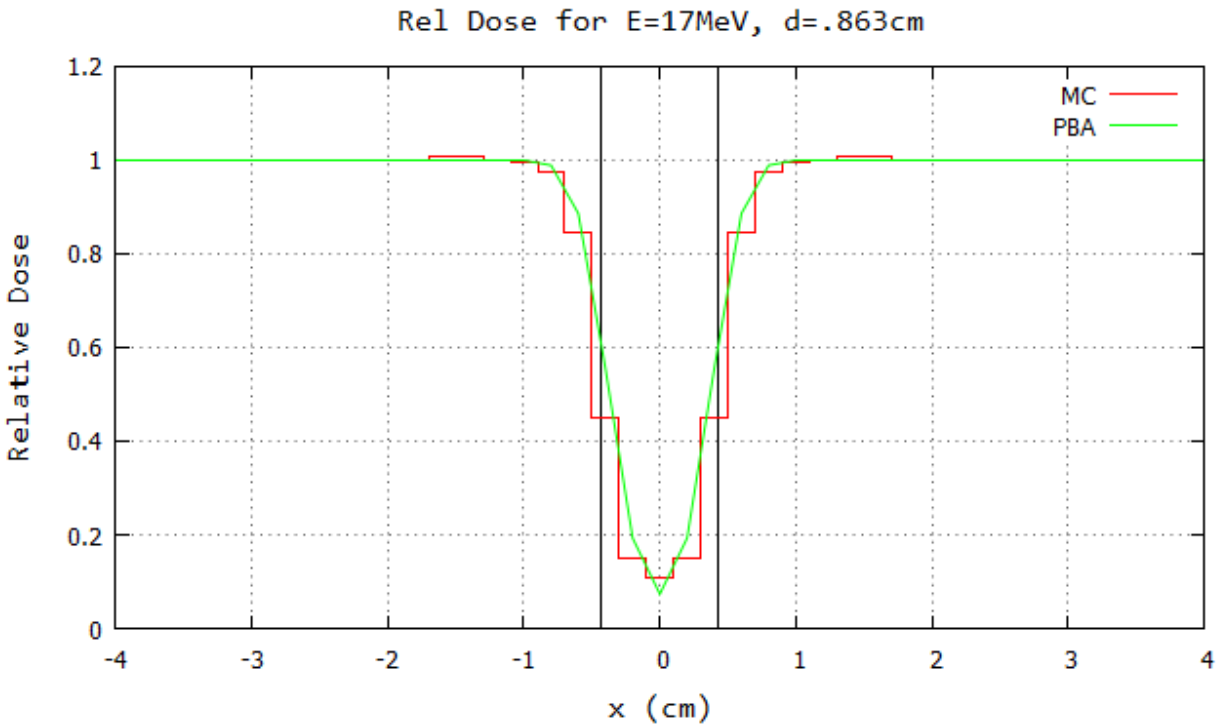
Figure 2.5: PBA/MC profiles comparisons for a monoenergetic 17 MeV beam with a central axis block of diameter d=0.863\text{cm} at depth z=0.5\text{cm} with air gap g=5.0\text{ cm} . (a) Relative intensity profile ( y=0 ) for Monte Carlo and pencil-beam algorithm calculations, and (b), zoomed in version for detail. Vertical black lines indicate the position of the block.
