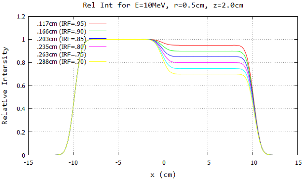
Figure 3.3: Profiles at y=0\text{cm} for 10 MeV, 20\times 20 half-blocked field ( r=0.5\text{cm} ), 100 cm SSD: z=0.5\text{cm} (top) and z=2.0\text{cm} (bottom). The computed island block diameter for 0.70, 0.75, 0.80, 0.85, 0.90, and 0.95 IRF values are listed in each plot's inserted key.
