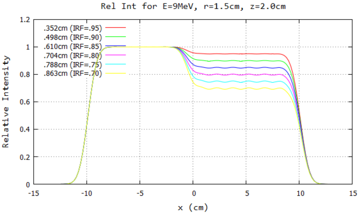
Figure B.45: Profile for 9 MeV and 103 cm SSD at y=0\text{cm} 20x20 half-blocked field. The computed island block diameter for 0.70, 0.75, 0.80, 0.85, 0.90, and 0.95 IRF values are listed in each plot's inserted key.
