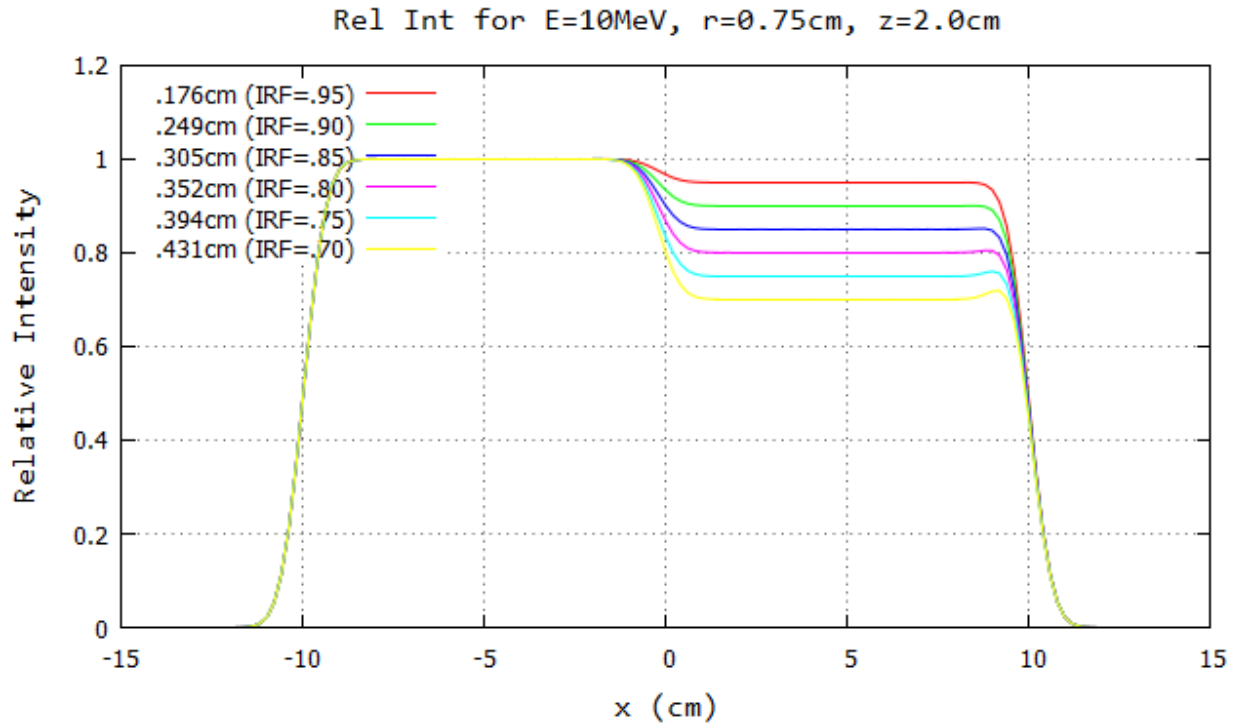
Figure B.12: Profile for 10 MeV and 100 cm SSD at y=0 cm 20x20 half-blocked field. The computed island block diameter for 0.70, 0.75, 0.80, 0.85, 0.90, and 0.95 IRF values are listed in each plot's inserted key.
