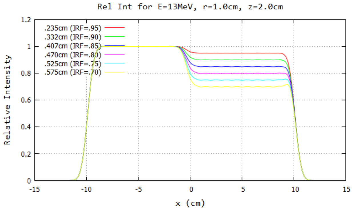
Figure B.58: Profile for 13 MeV and 103 cm SSD at y=0\text{cm} 20x20 half-blocked field. The computed island block diameter for 0.70, 0.75, 0.80, 0.85, 0.90, and 0.95 IRF values are listed in each plot's inserted key.
